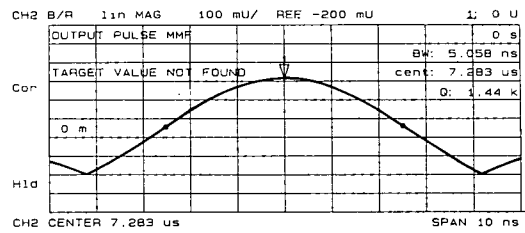
(b) Measuring Pulse Dispersion on a 1.5 km Fiber Optic Cable
