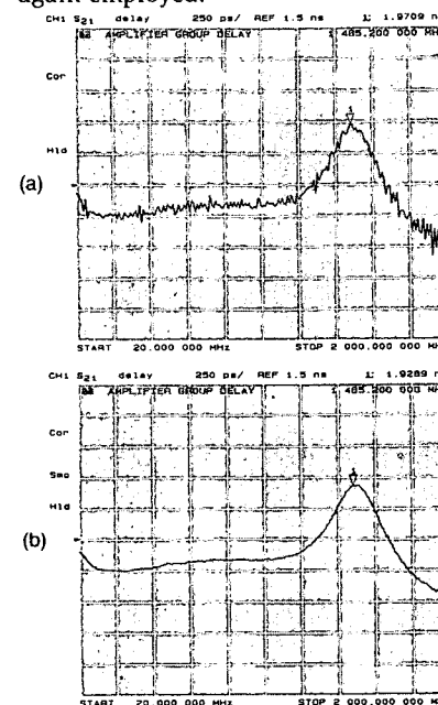
Figure 9. Group delay measurement: (a) with minimum aperture and (b) with increased aperture.
