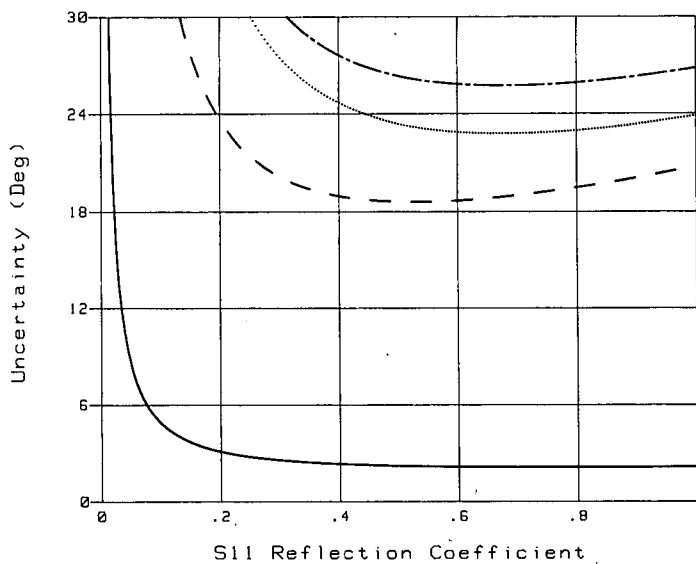
Figure 6. Total Reflection Phase Uncertainty
