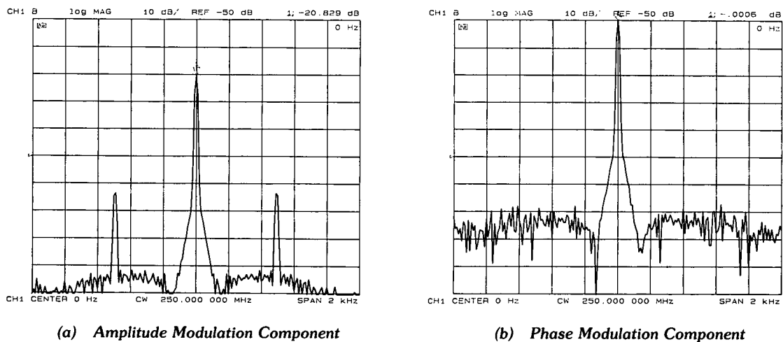
Figure 8-19. Separating the Amplitude and Phase Components of DUT-Induced Modulation
