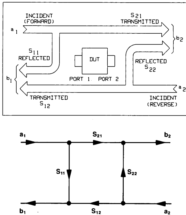
Figure 4-3. S-Parameters of a Two-Port Device
