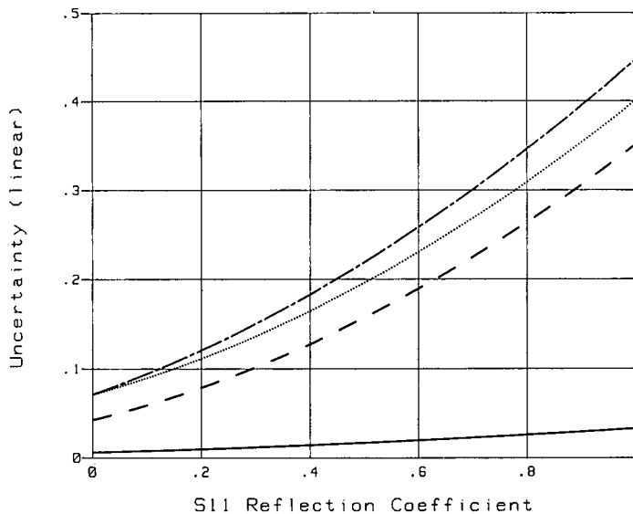
Figure 5. Total Reflection Magnitude Uncertainty
