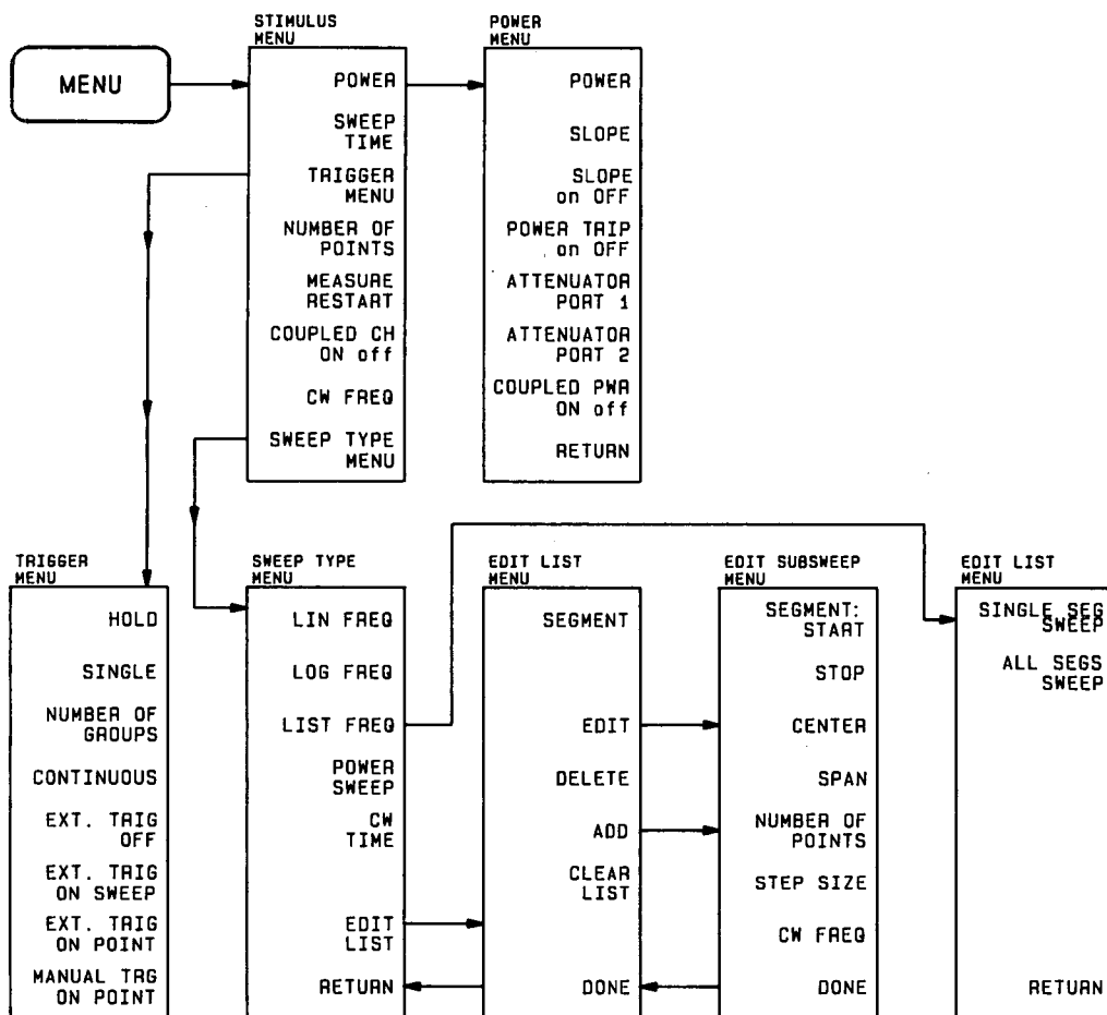
Figure 3-2. Softkey Menus Accessed from the [MENU] Key
